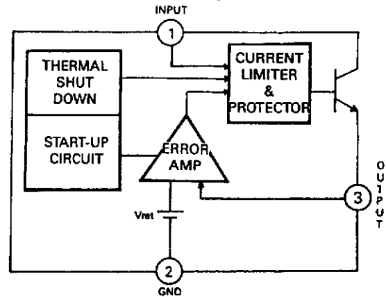
2. Block Diagram
